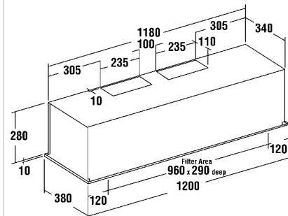
ECH-1200-2-T/B
